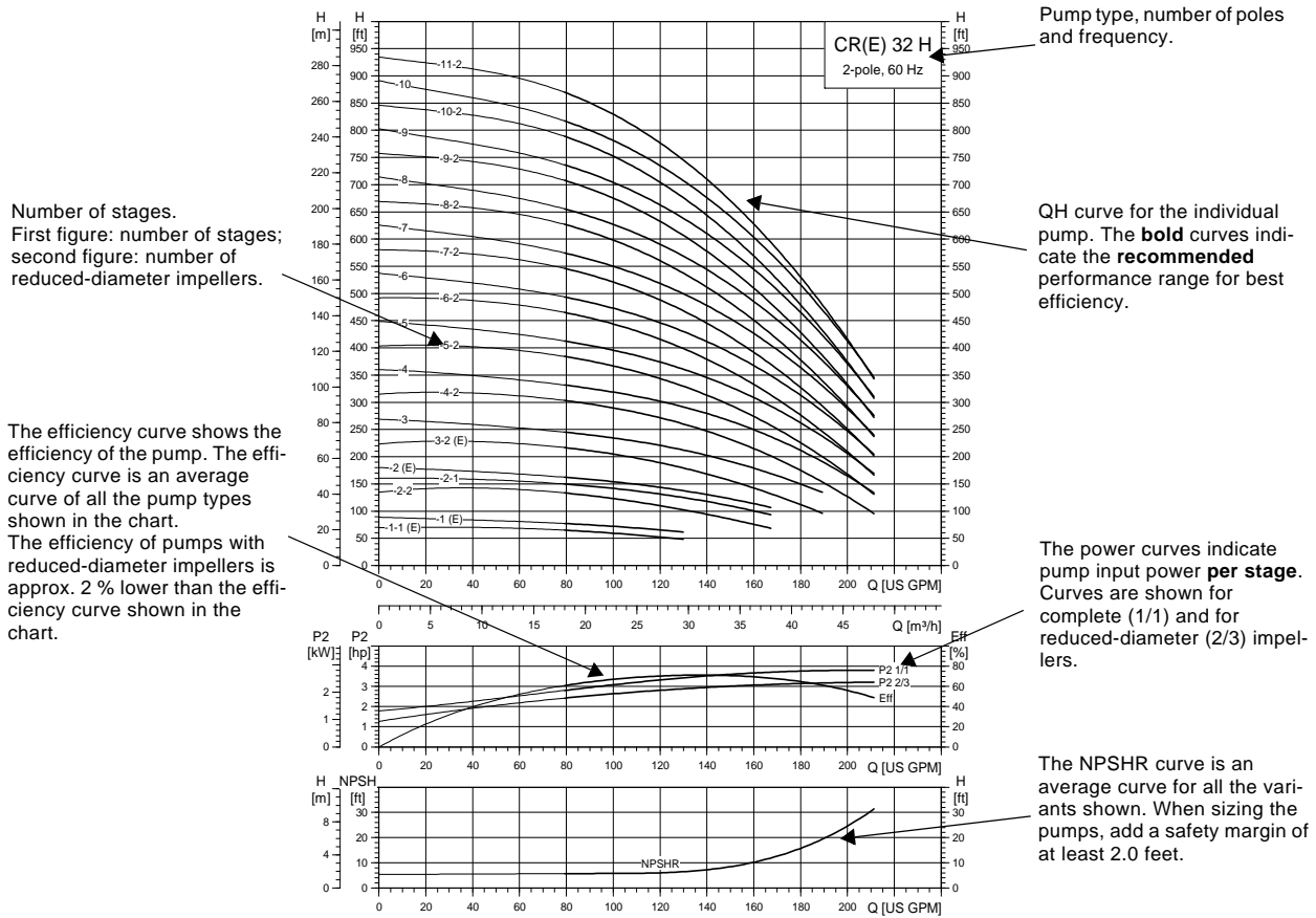
Fig. 29 How to read the curve charts
