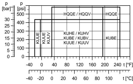
Fig. 18 Operating range of standard shaft seals for CR 32 H to CR 90 H
