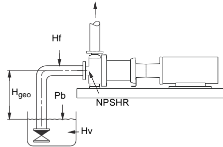
Fig. 20 Sizing data
