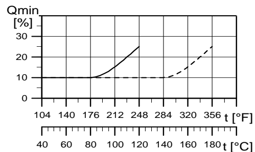
Fig. 30 Minimum flow rate
