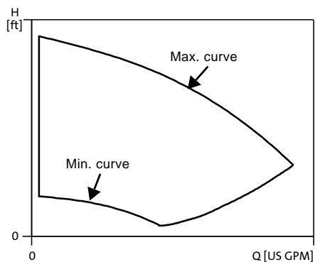
Fig. 23 Min. and max. performance curves
