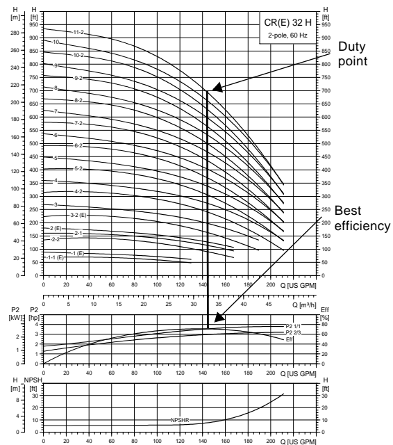
Fig. 21 Example of a CR pump's duty point
