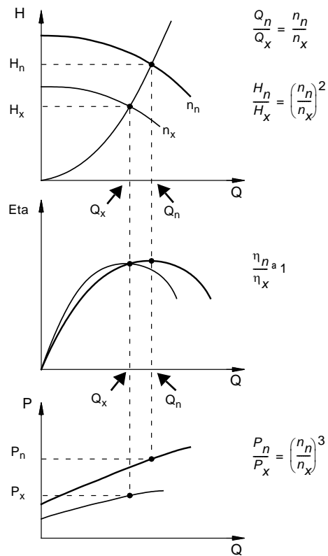
Fig. 24 Affinity equations
