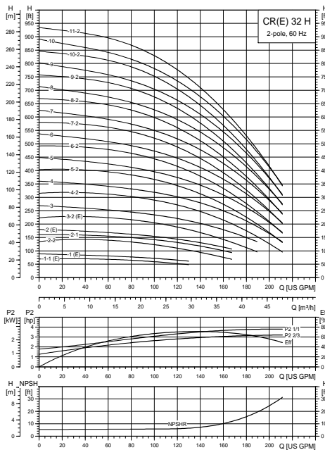
Fig. 19 Example of a curve chart
