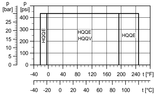
Fig. 17 Operating range of standard shaft seals for CR 1s H to CR 20 H
