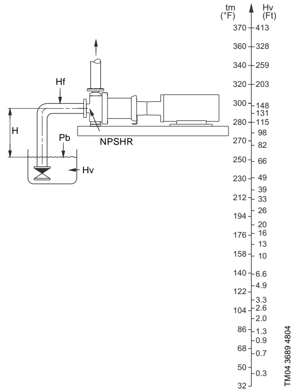
Fig. 28 Minimum inlet pressure - NPSHR
