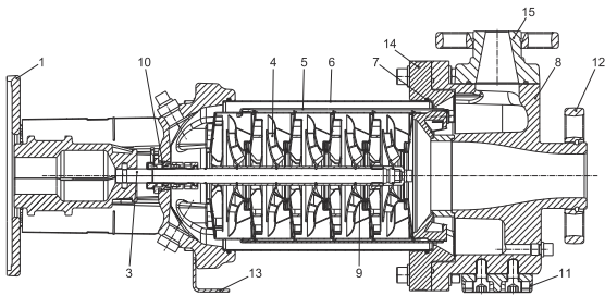
Fig. 14 Sectional drawing
