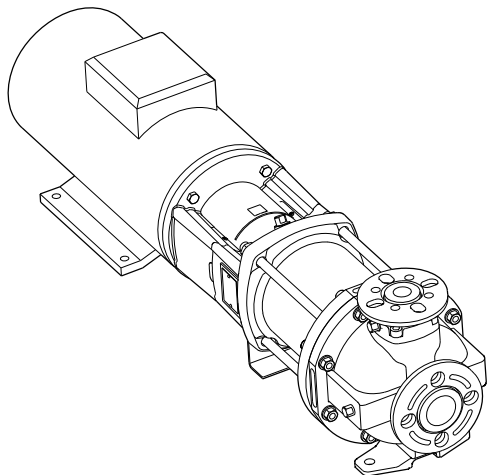
Fig. 25 CR-H pump
