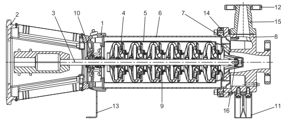
Fig. 16 Sectional drawing
